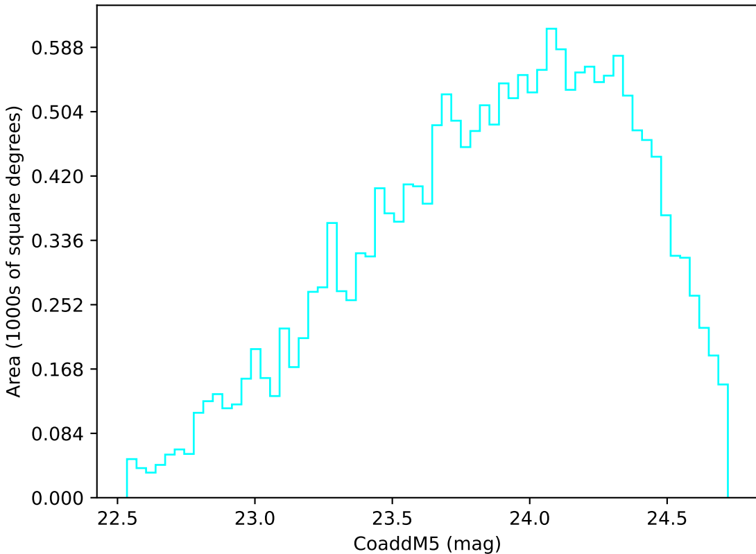
ddf_half_v3.4_10yrs Yr 3-4 u band: CoaddM5
