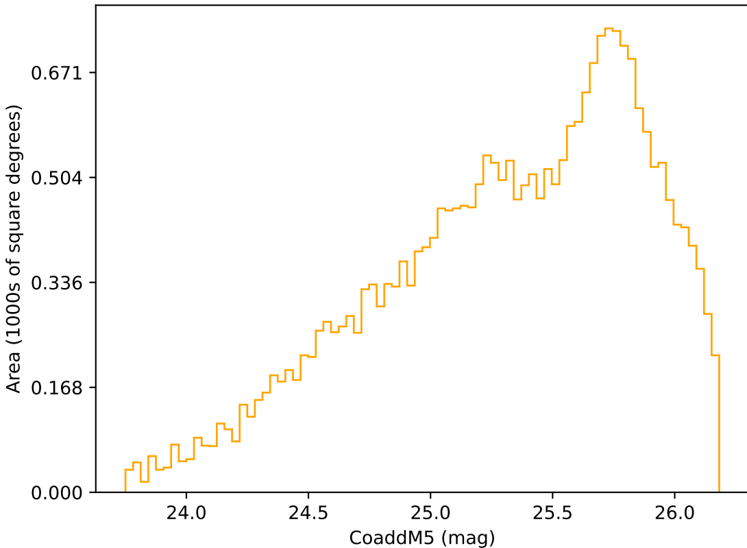
ddf_half_v3.4_10yrs Yr 3-4 r band: CoaddM5
