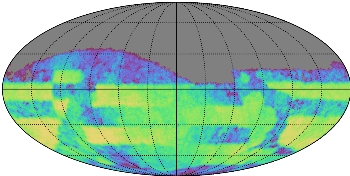
ddf_half_v3.4_10yrs Yr 3-4 i band: CoaddM5
