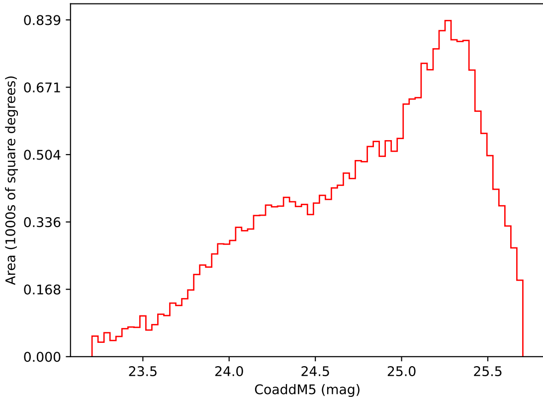
ddf_half_v3.4_10yrs Yr 3-4 i band: CoaddM5
