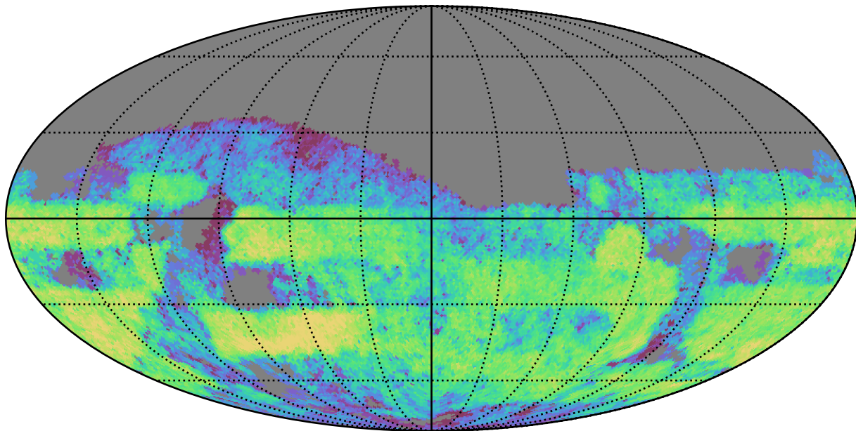
ddf_half_v3.4_10yrs Yr 3-4 g band: CoaddM5
