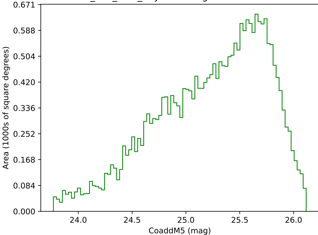
ddf_half_v3.4_10yrs Yr 3-4 g band: CoaddM5
