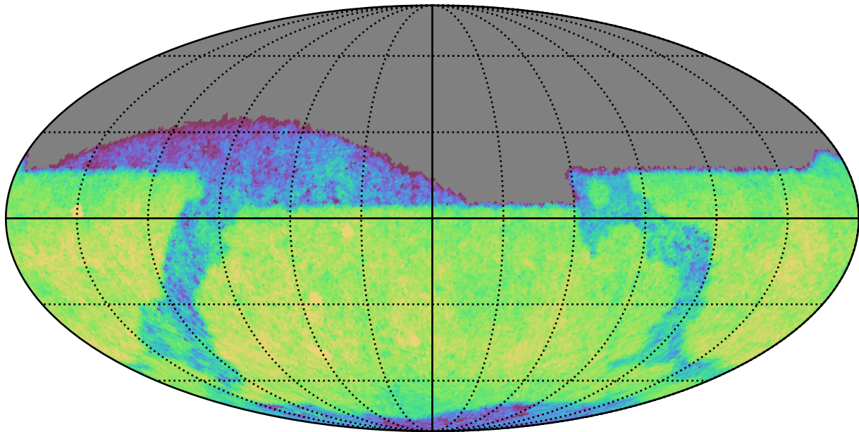
ddf_half_v3.4_10yrs Yr 1 z band: CoaddM5
