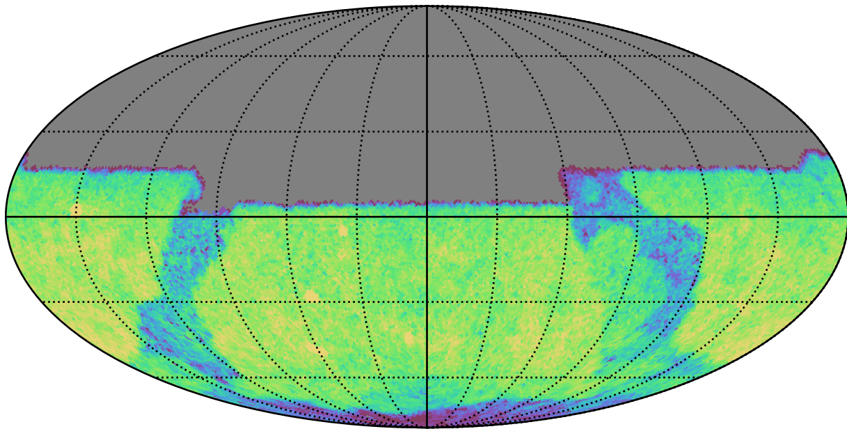
ddf_half_v3.4_10yrs Yr 1 y band: CoaddM5
