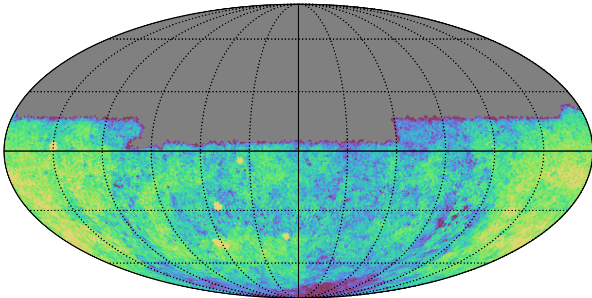
ddf_half_v3.4_10yrs Yr 1 u band: CoaddM5
