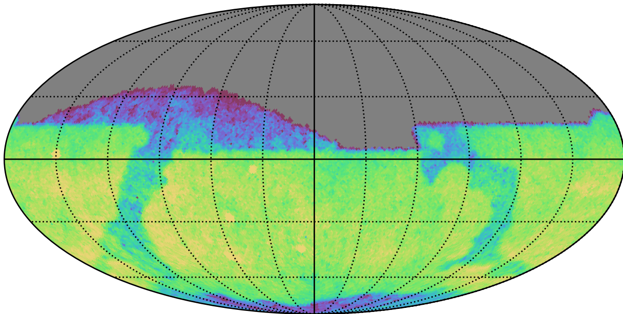
ddf_half_v3.4_10yrs Yr 1 r band: CoaddM5
