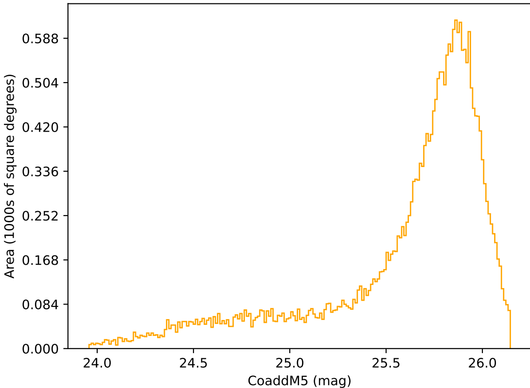
ddf_half_v3.4_10yrs Yr 1 r band: CoaddM5
