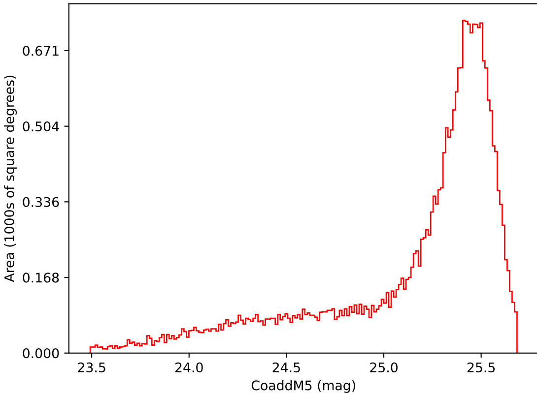
ddf_half_v3.4_10yrs Yr 1 i band: CoaddM5
