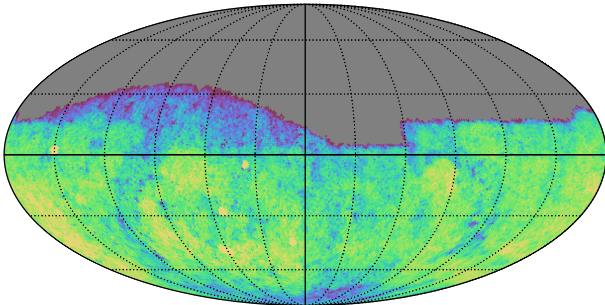
ddf_half_v3.4_10yrs Yr 1 g band: CoaddM5
