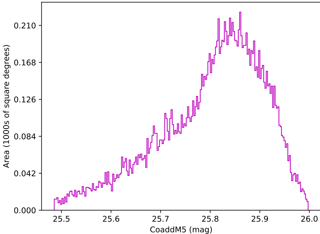
ddf_half_v3.4_10yrs WFD z band: CoaddM5
