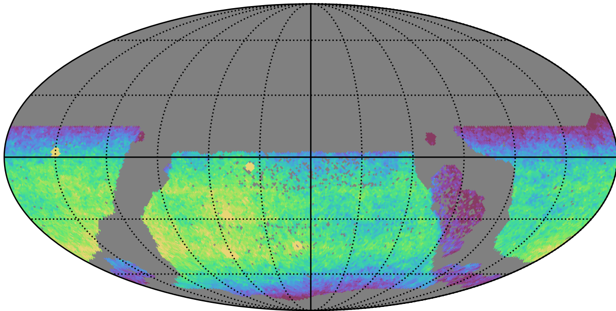
ddf_half_v3.4_10yrs WFD y band: CoaddM5
