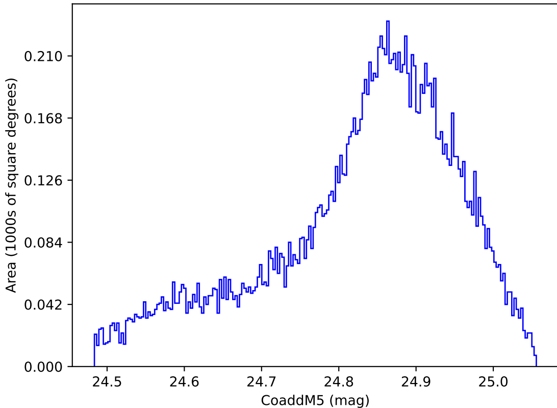
ddf_half_v3.4_10yrs WFD y band: CoaddM5
