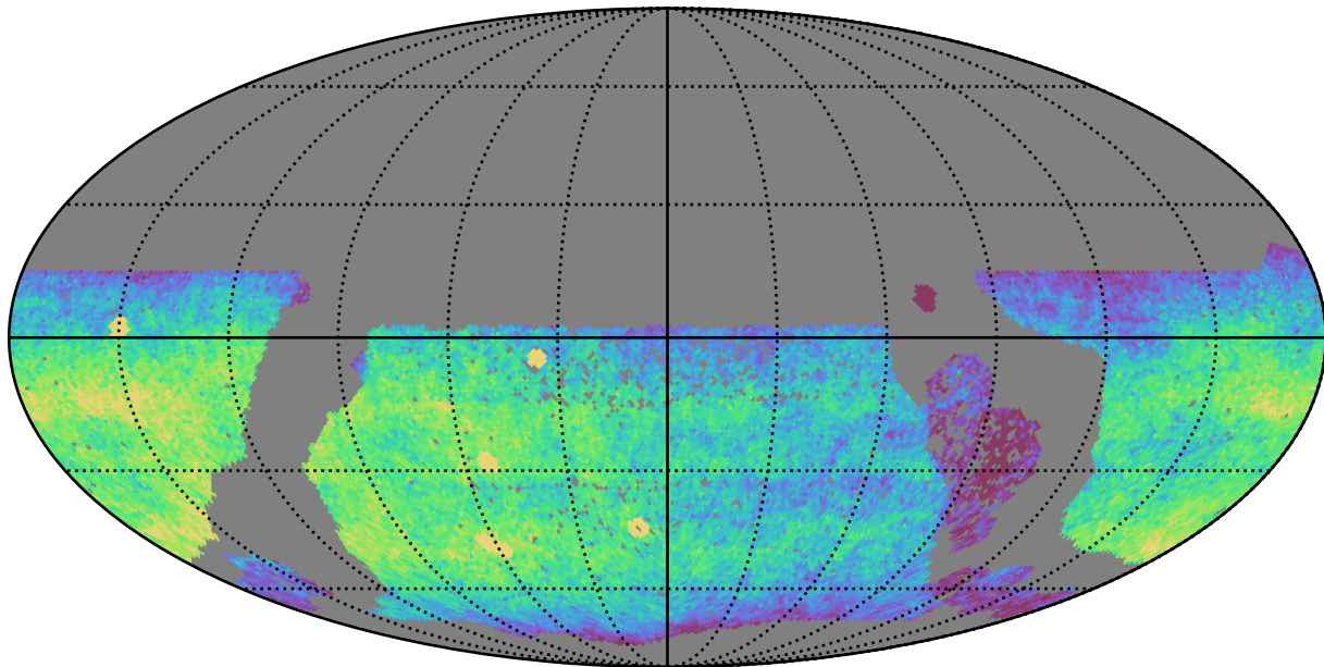
ddf_half_v3.4_10yrs WFD u band: CoaddM5
