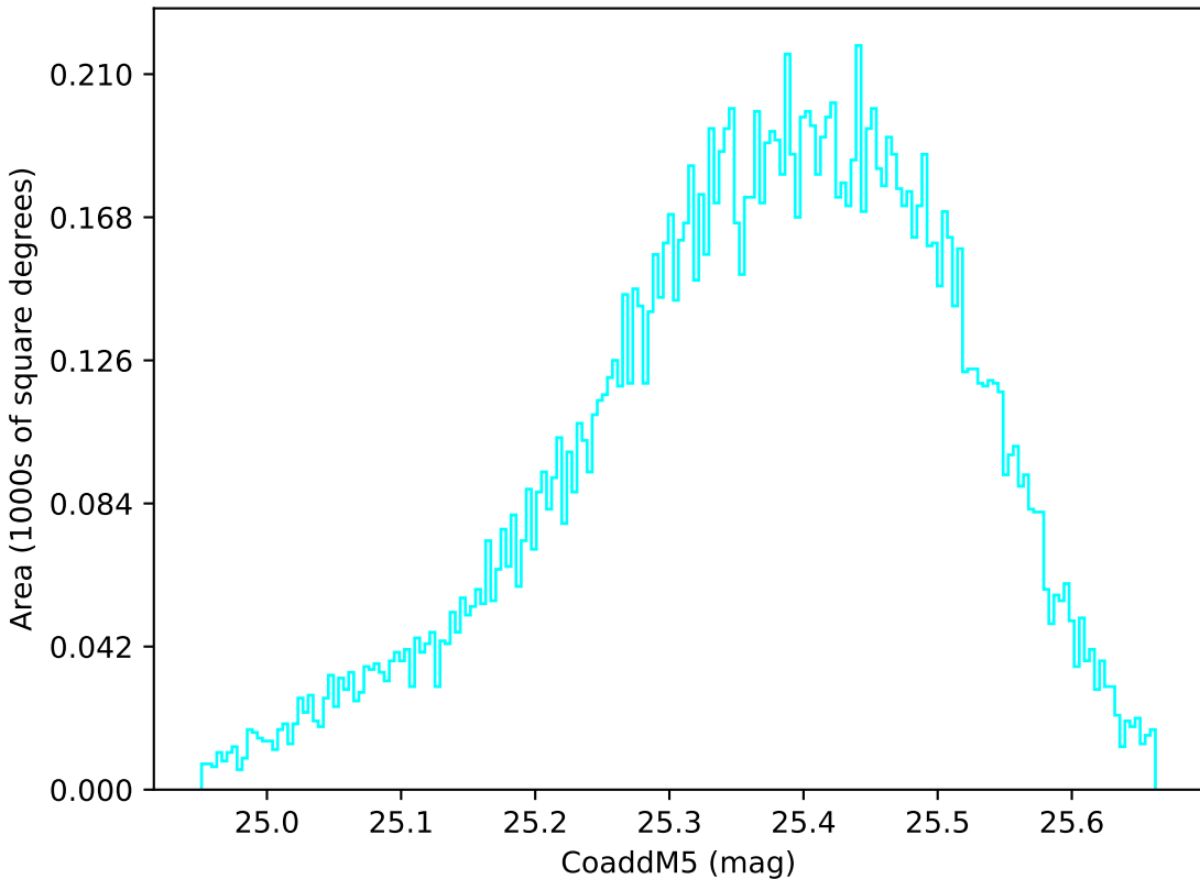
ddf_half_v3.4_10yrs WFD u band: CoaddM5
