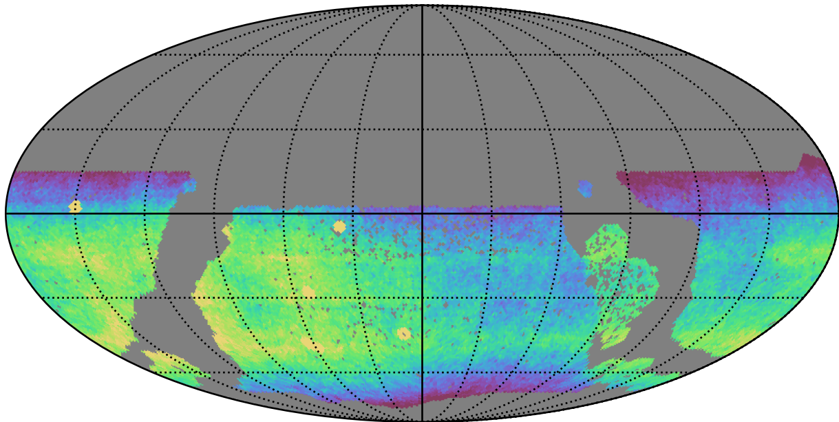
ddf_half_v3.4_10yrs WFD r band: CoaddM5
