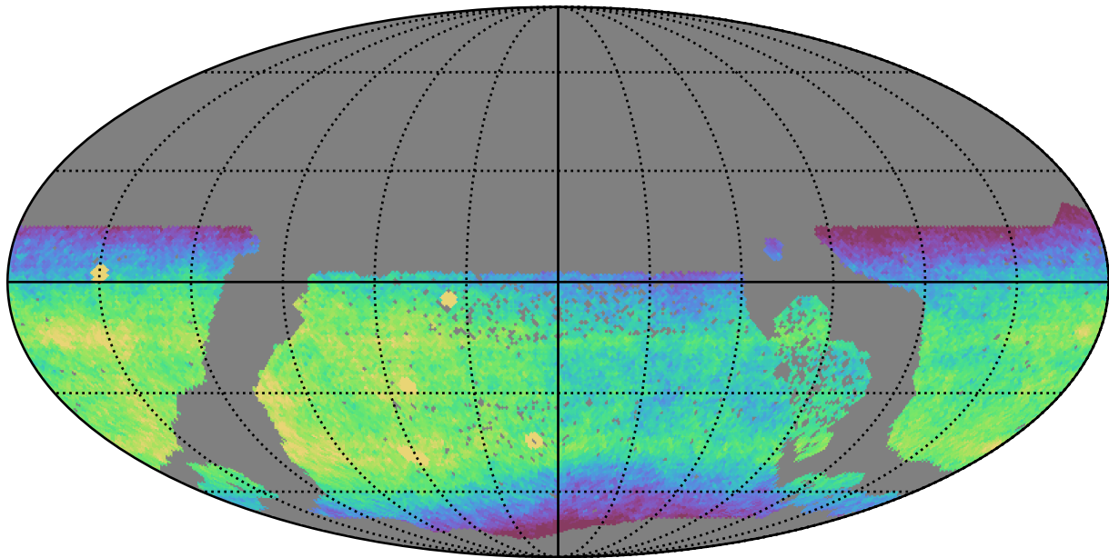
ddf_half_v3.4_10yrs WFD i band: CoaddM5
