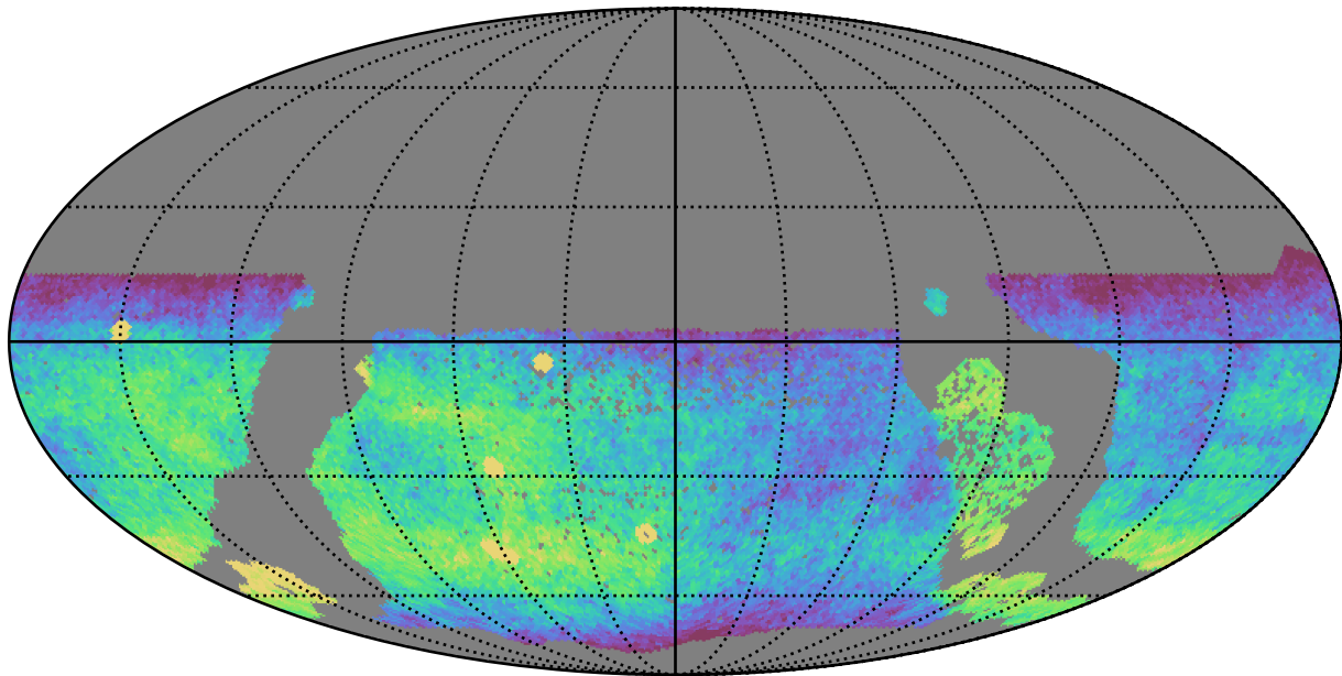
ddf_half_v3.4_10yrs WFD g band: CoaddM5
