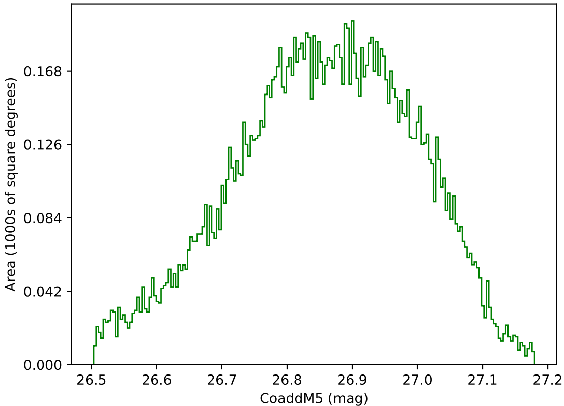
ddf_half_v3.4_10yrs WFD g band: CoaddM5
