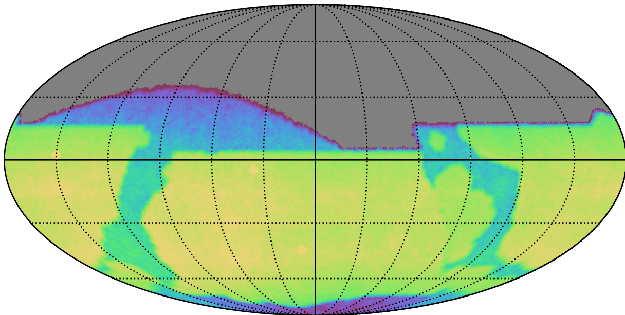
ddf_half_v3.4_10yrs All sky z band: CoaddM5
