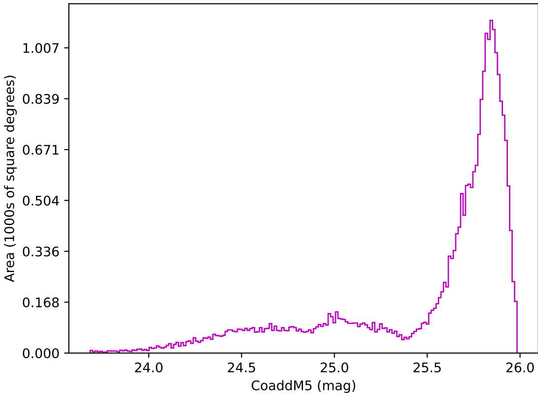
ddf_half_v3.4_10yrs All sky z band: CoaddM5
