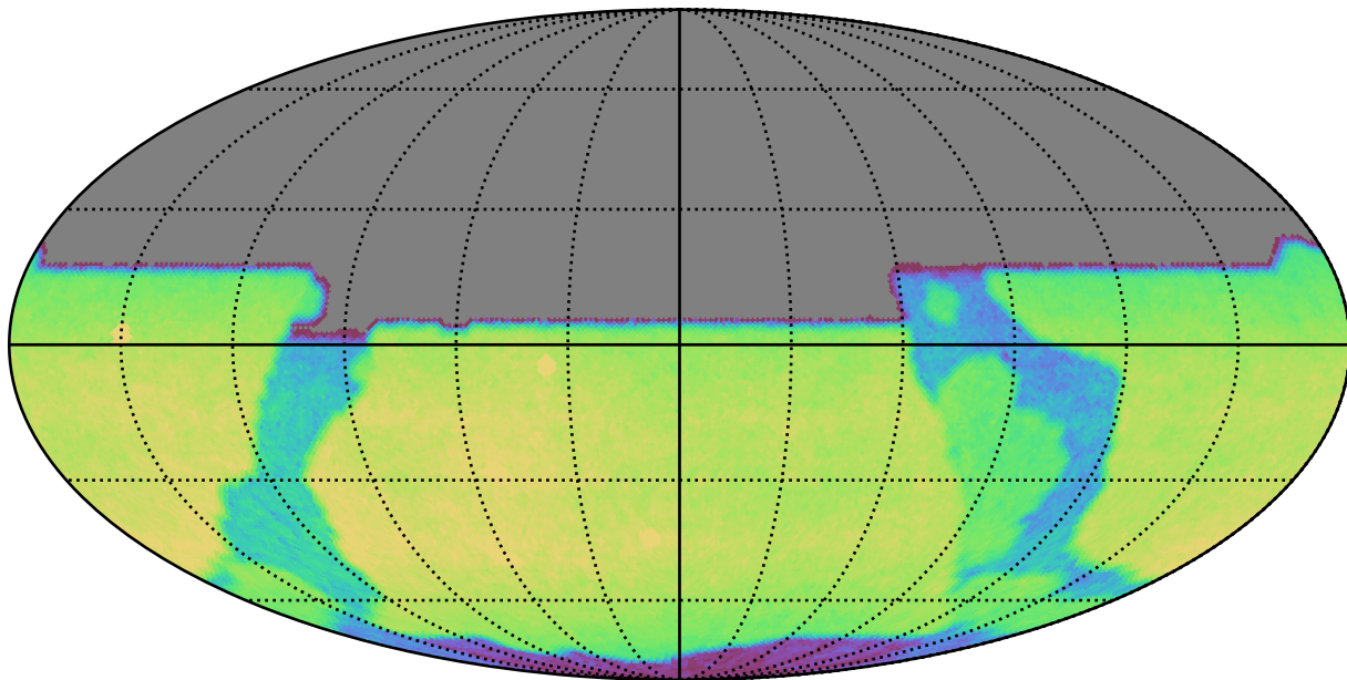
ddf_half_v3.4_10yrs All sky y band: CoaddM5
