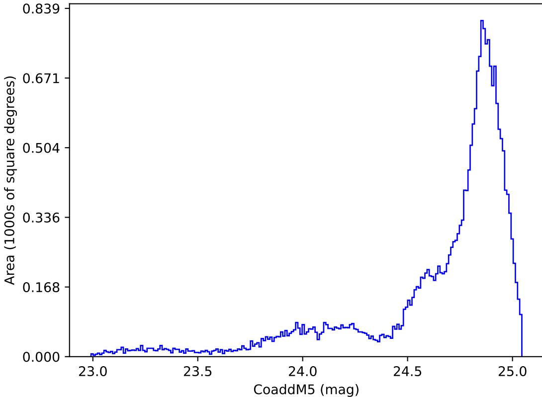
ddf_half_v3.4_10yrs All sky y band: CoaddM5
