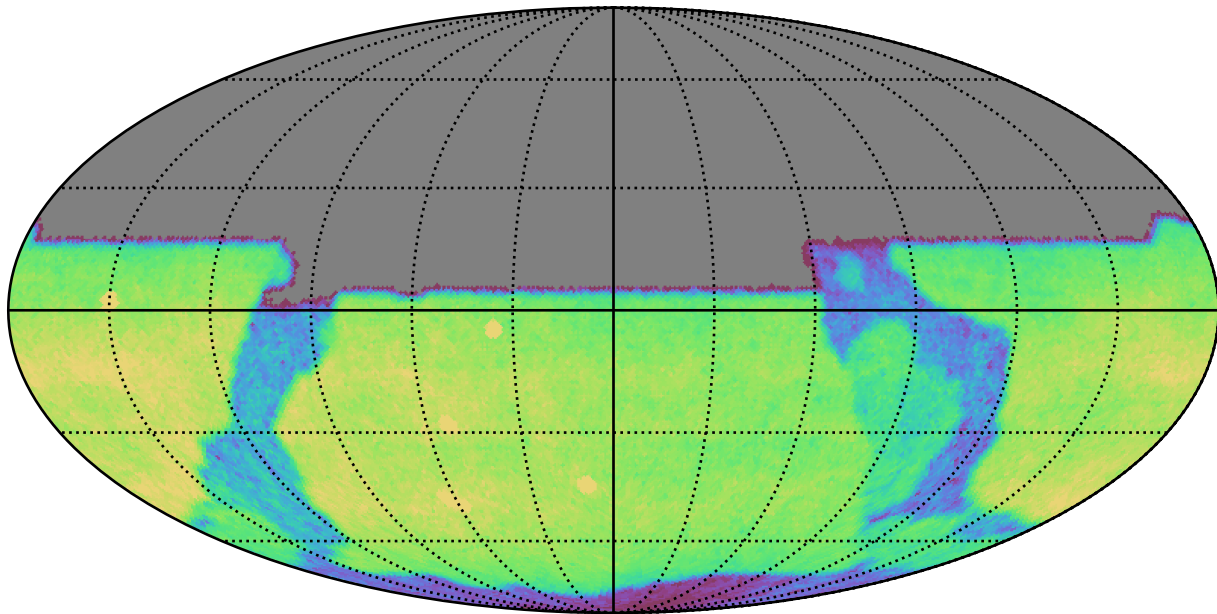
ddf_half_v3.4_10yrs All sky u band: CoaddM5
