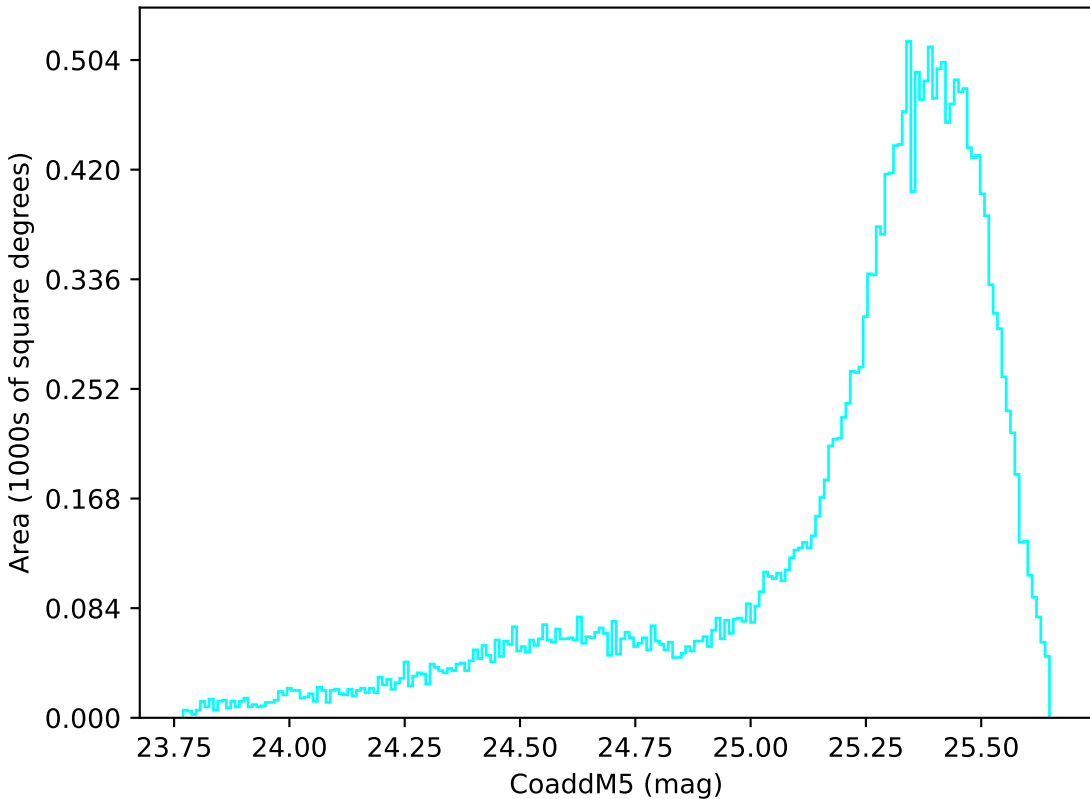
ddf_half_v3.4_10yrs All sky u band: CoaddM5
