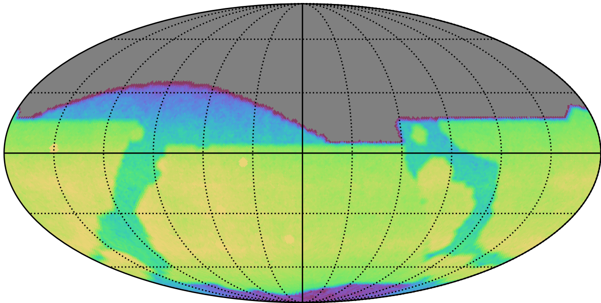
ddf_half_v3.4_10yrs All sky r band: CoaddM5
