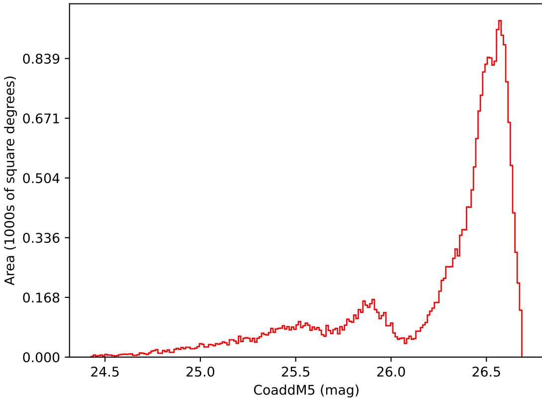
ddf_half_v3.4_10yrs All sky i band: CoaddM5
