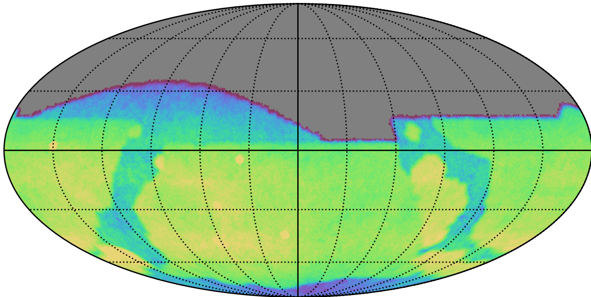
ddf_half_v3.4_10yrs All sky g band: CoaddM5
