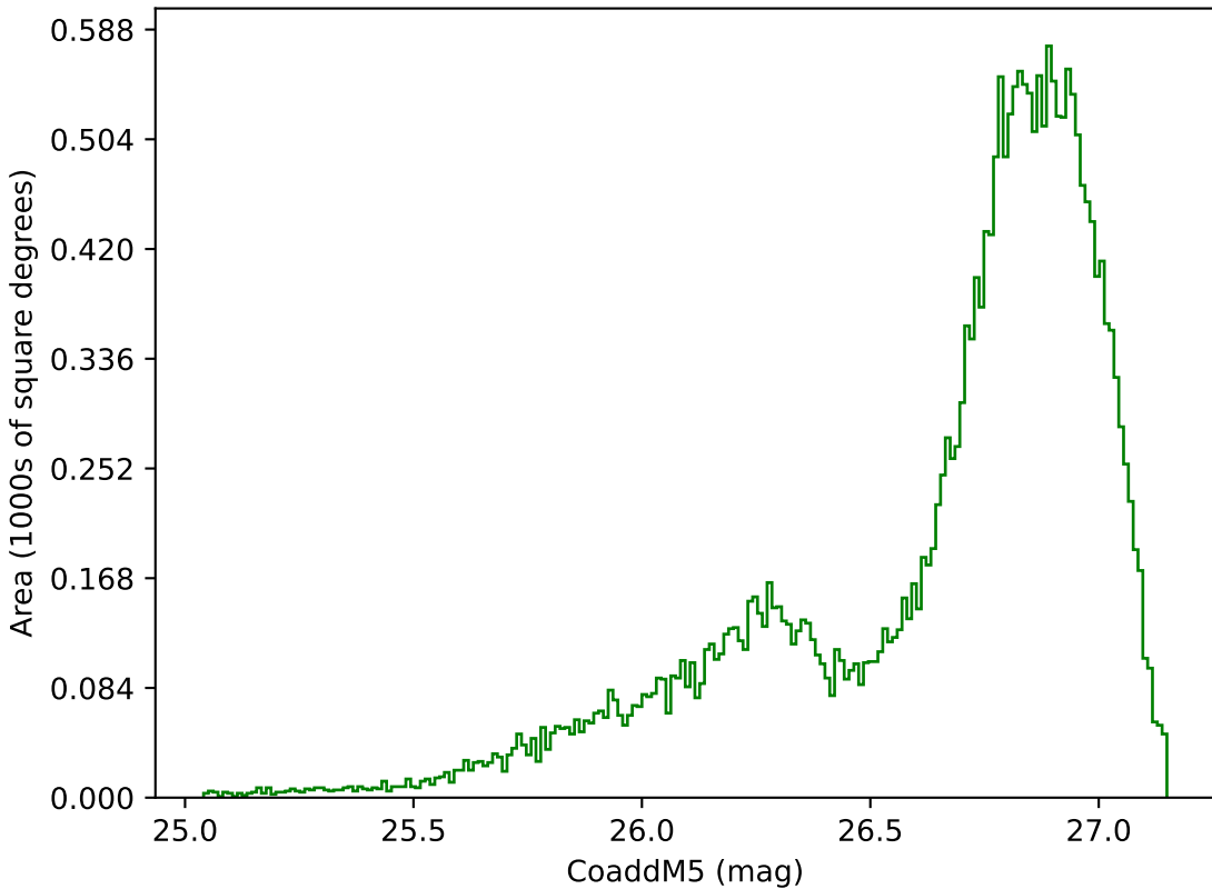
ddf_half_v3.4_10yrs All sky g band: CoaddM5
