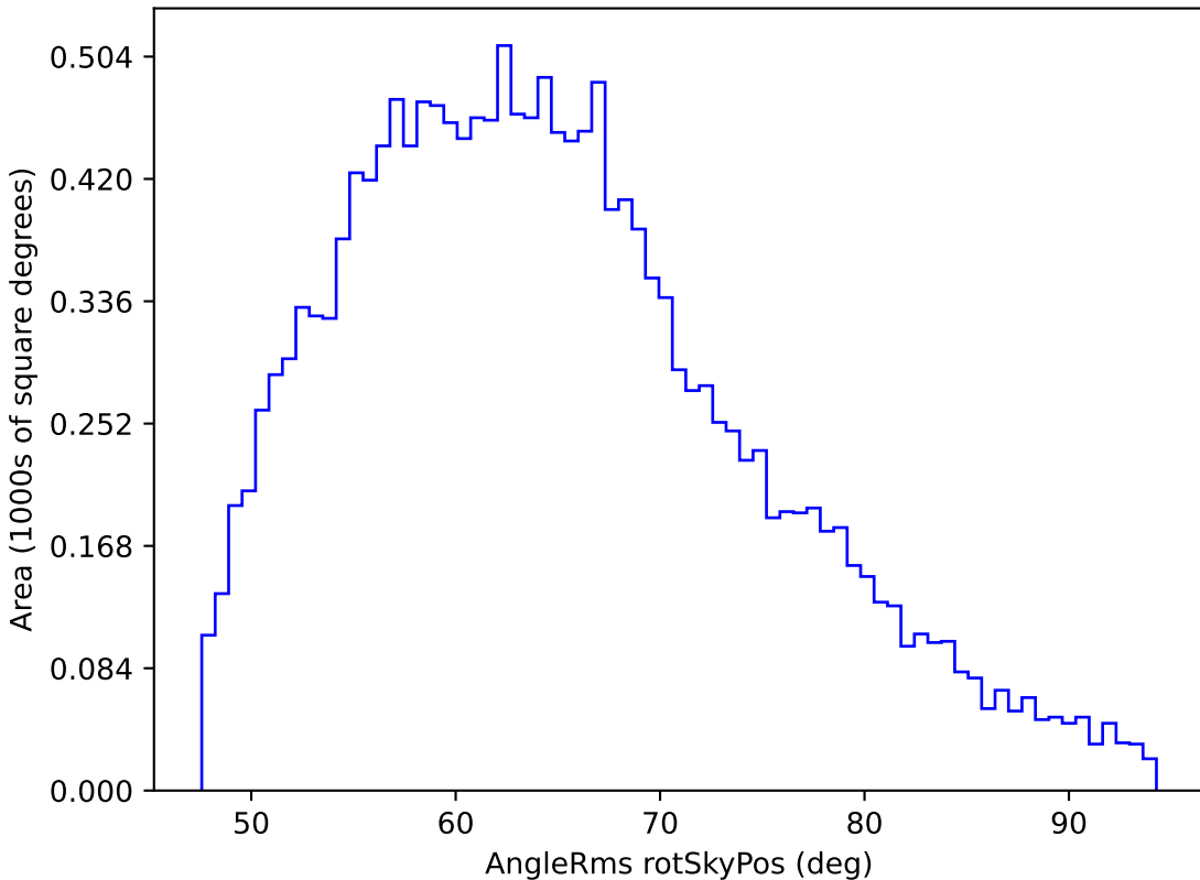
ddf_half_v3.4_10yrs WFD z band: AngleRms rotSkyPos
