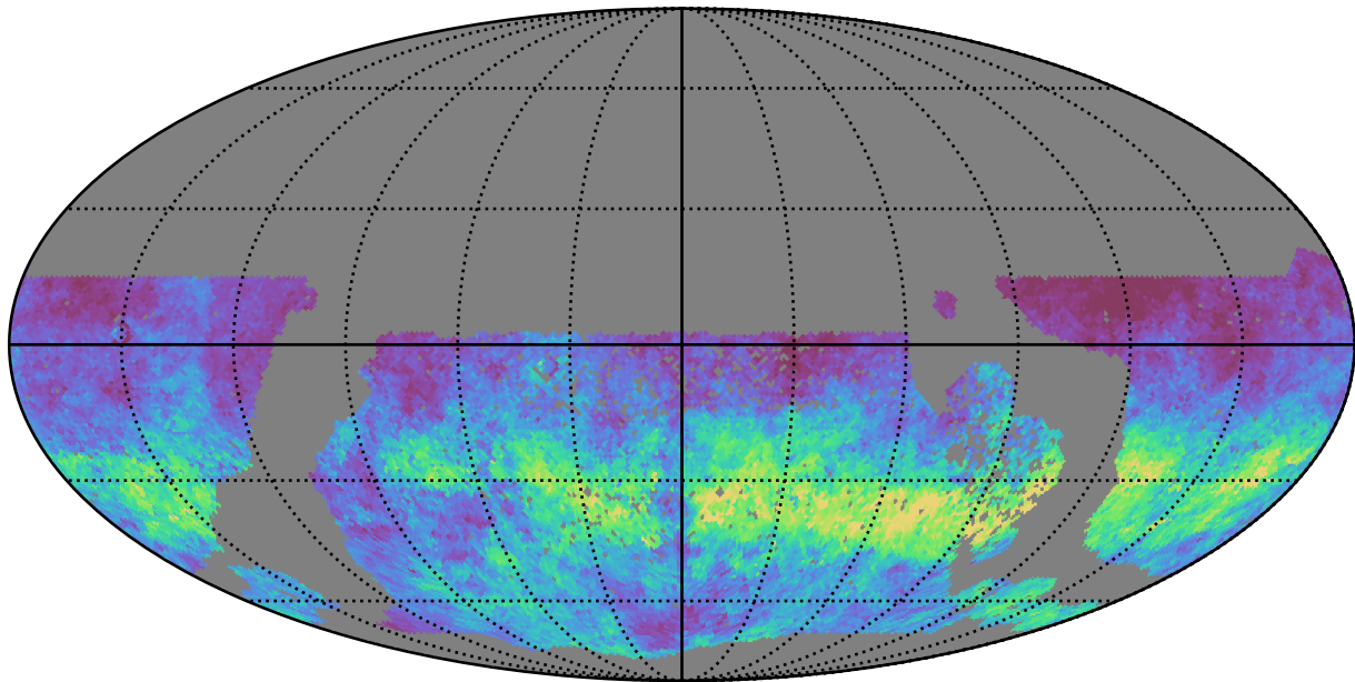
ddf_half_v3.4_10yrs WFD u band: AngleRms rotSkyPos
