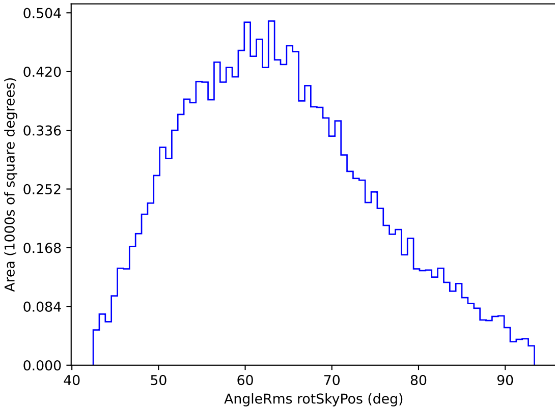
ddf_half_v3.4_10yrs WFD u band: AngleRms rotSkyPos
