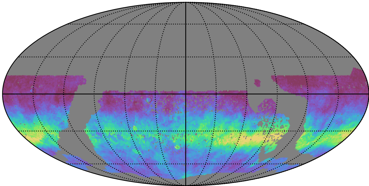
ddf_half_v3.4_10yrs WFD r band: AngleRms rotSkyPos
