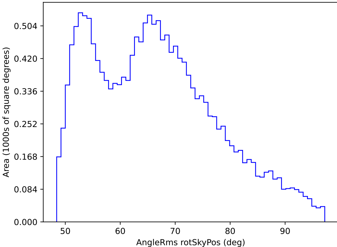
ddf_half_v3.4_10yrs WFD r band: AngleRms rotSkyPos
