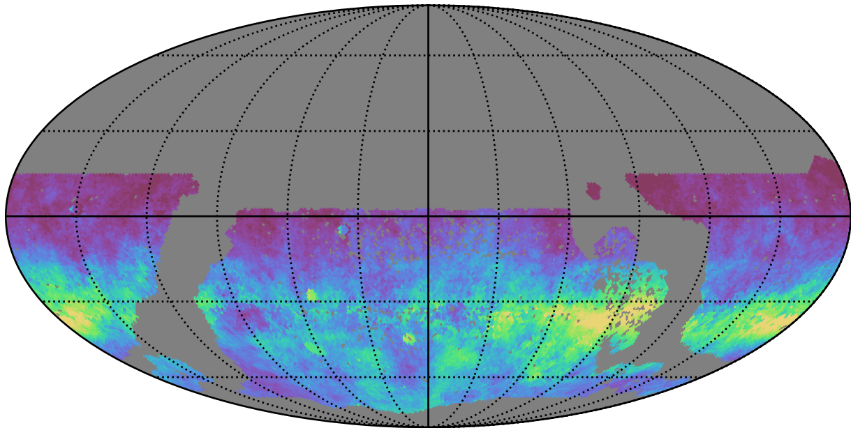
ddf_half_v3.4_10yrs WFD i band: AngleRms rotSkyPos
