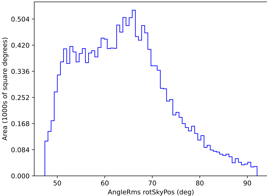
ddf_half_v3.4_10yrs WFD i band: AngleRms rotSkyPos
