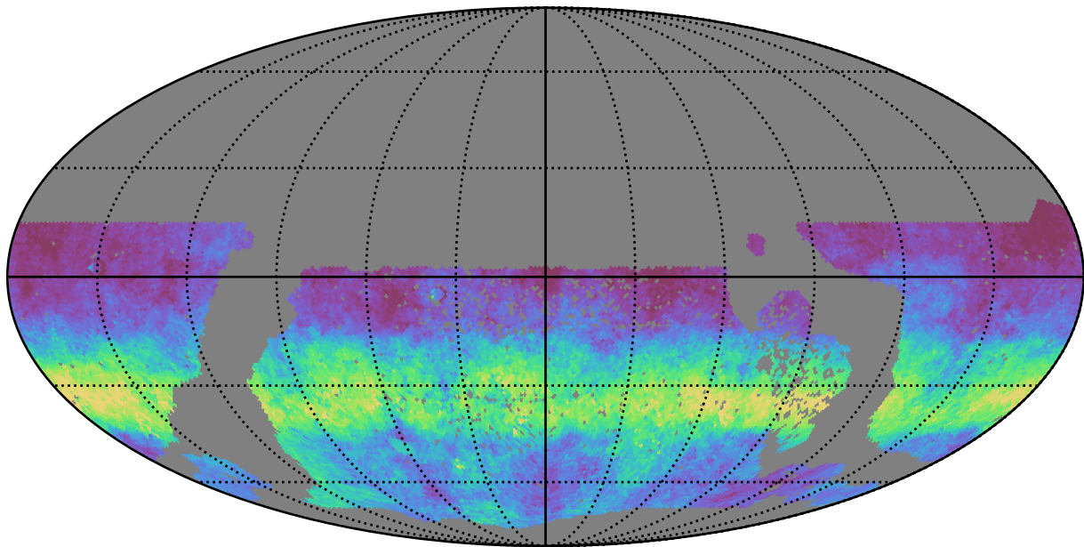
ddf_half_v3.4_10yrs WFD g band: AngleRms rotSkyPos
