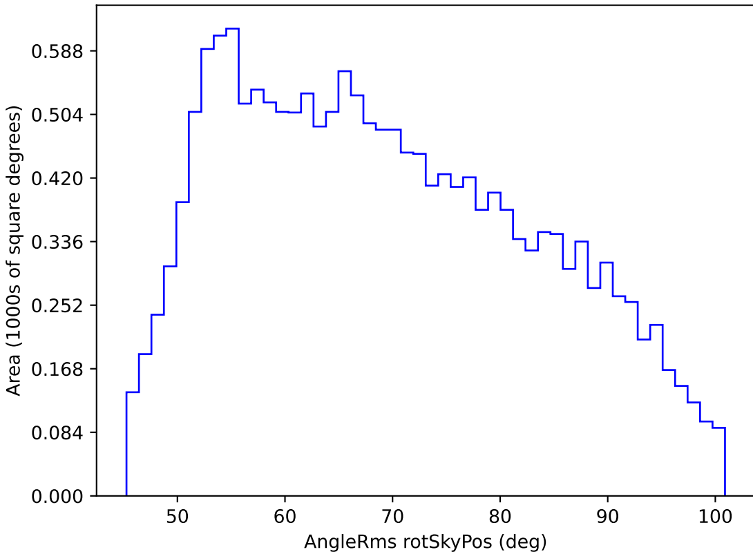
ddf_half_v3.4_10yrs WFD g band: AngleRms rotSkyPos
