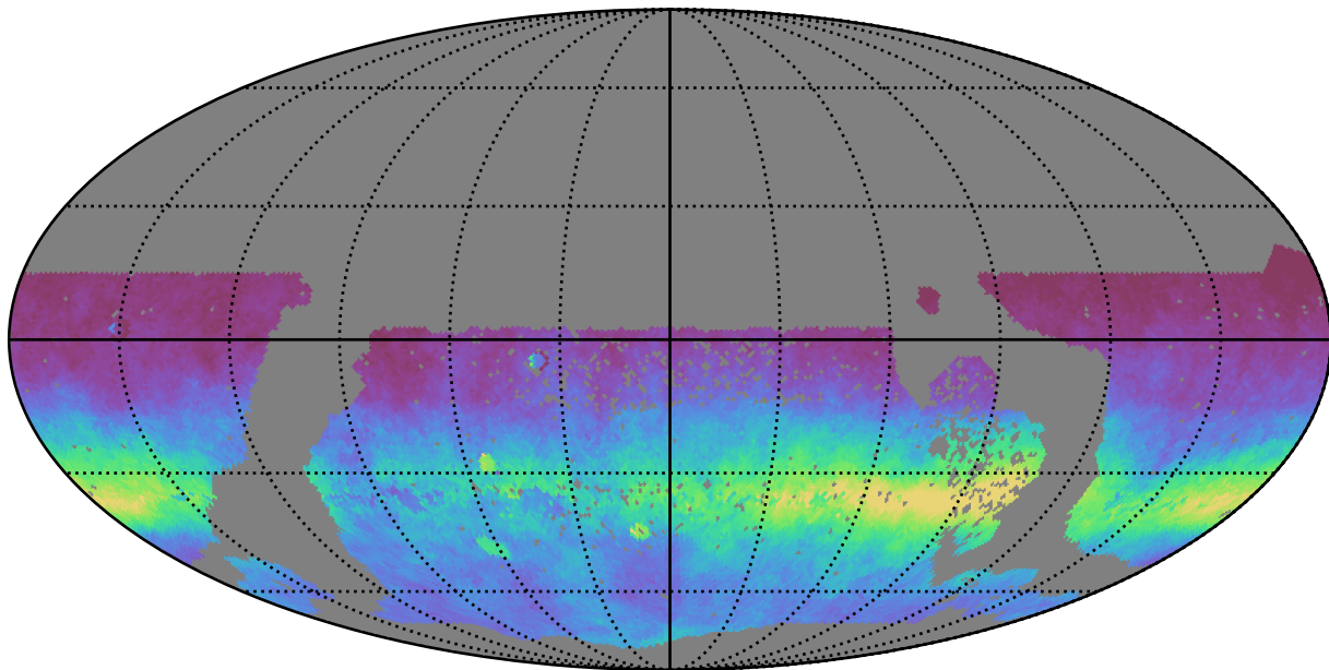
ddf_half_v3.4_10yrs WFD all bands: AngleRms rotSkyPos
