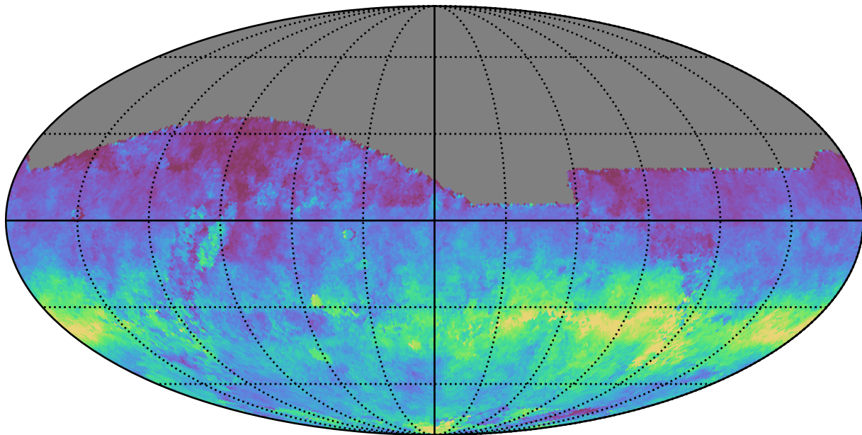
ddf_half_v3.4_10yrs All sky z band: AngleRms rotSkyPos
