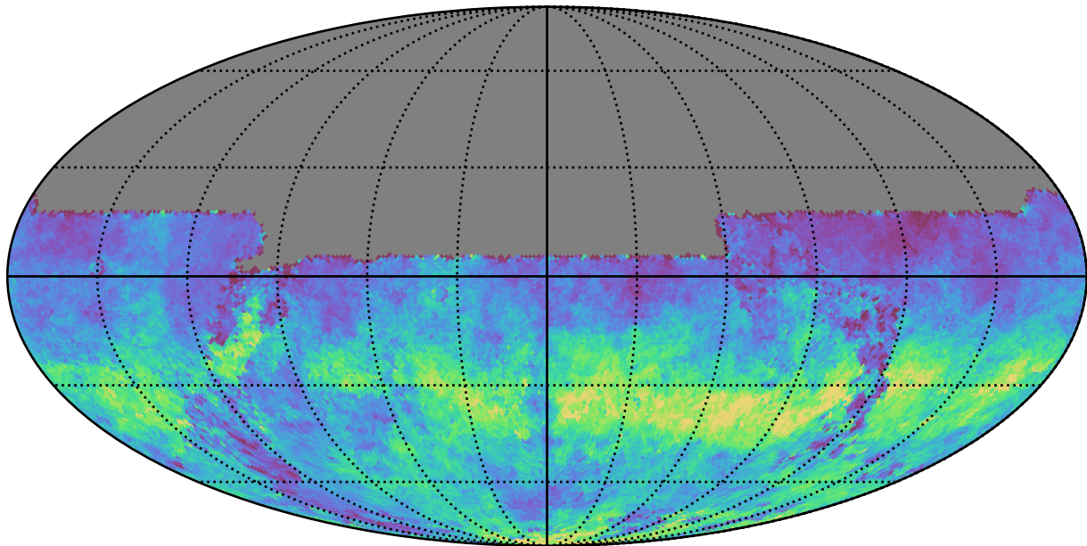
ddf_half_v3.4_10yrs All sky u band: AngleRms rotSkyPos
