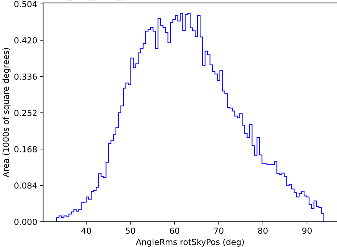
ddf_half_v3.4_10yrs All sky u band: AngleRms rotSkyPos
