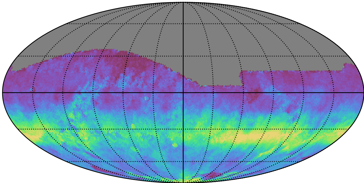
ddf_half_v3.4_10yrs All sky r band: AngleRms rotSkyPos
