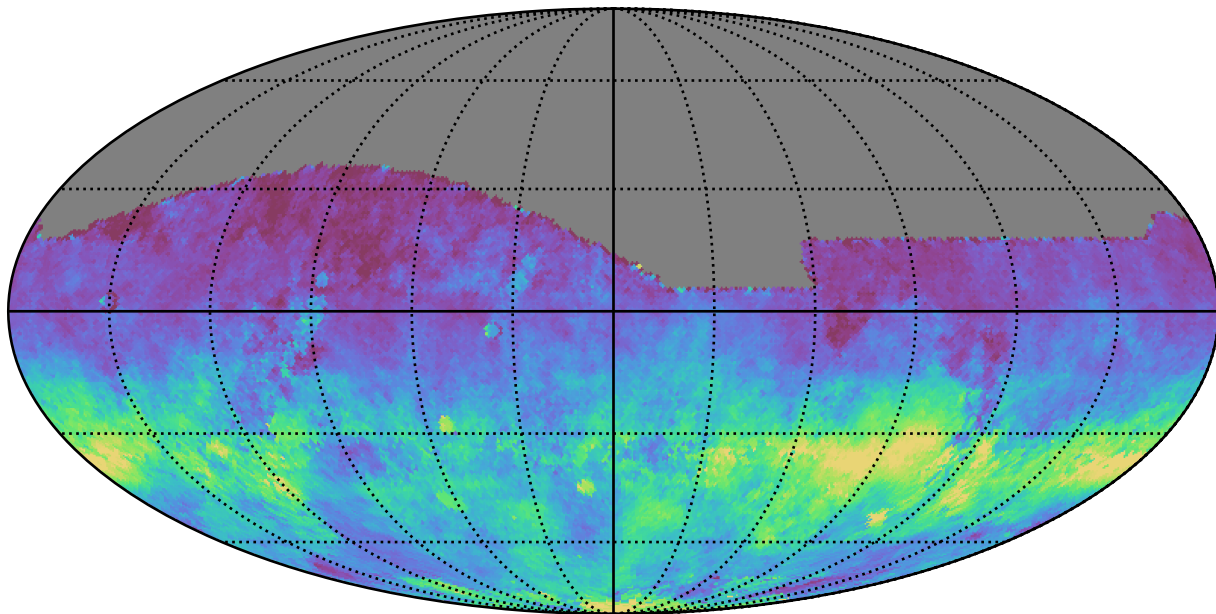
ddf_half_v3.4_10yrs All sky i band: AngleRms rotSkyPos
