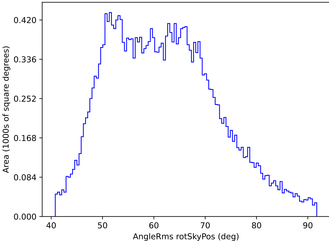
ddf_half_v3.4_10yrs All sky i band: AngleRms rotSkyPos
