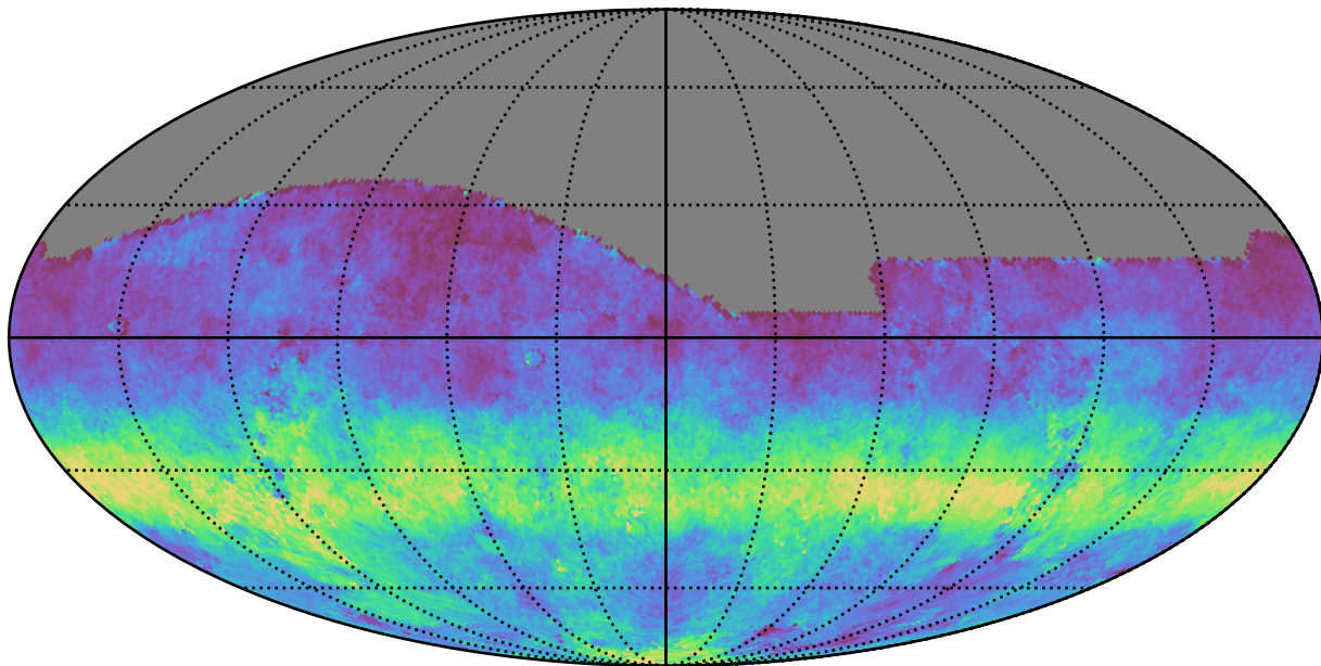
ddf_half_v3.4_10yrs All sky g band: AngleRms rotSkyPos
