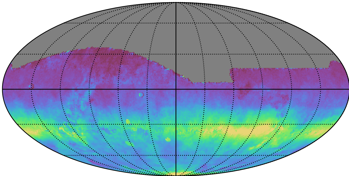
ddf_half_v3.4_10yrs All sky all bands: AngleRms rotSkyPos
